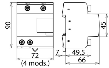
Dimension drawing DCB YPV 1200
